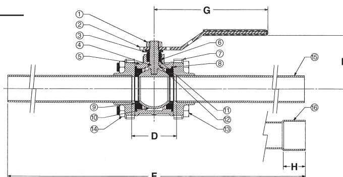
CS-595-YX/CS-595-YX-EC
