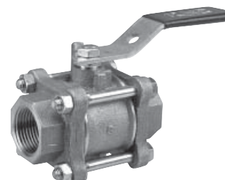
T-595-Y-SS Threaded
