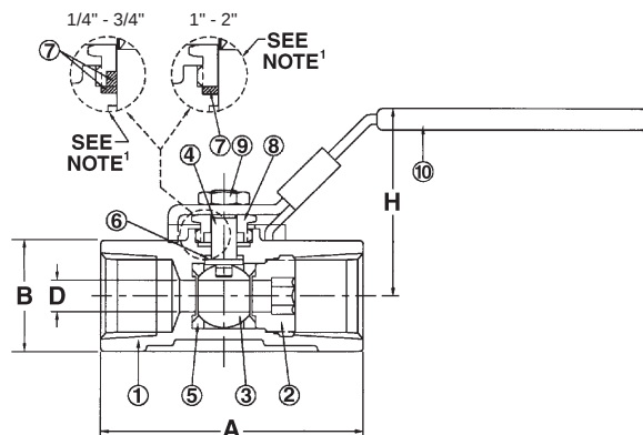
T-560-S6-R-66-LL
